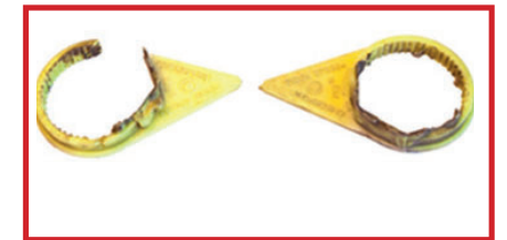
Indicators have melted = overheating problem Témoins fondus = surchauffe
